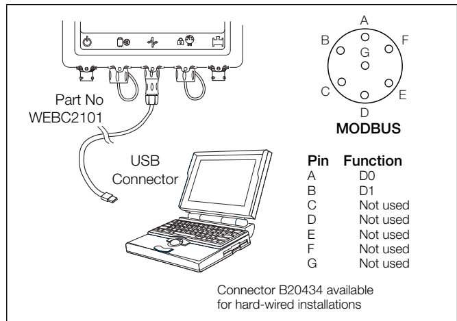
MODBUS connection
