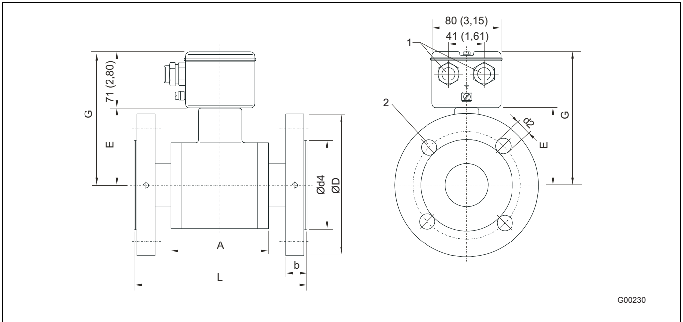
Fig. 32: Dimensions in mm (inch) 1 Cable gland M20 x 1.5 or NPT 2 Number of holes N
