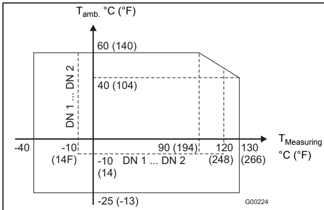
Fig. 27: Temperature graph
