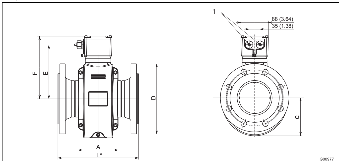
Fig. 22: Dimensions in mm (inch)
