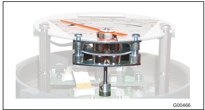
Fig. 9: Standard eddy-current brake
