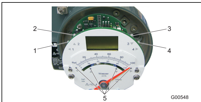
Fig. 12: Display with control buttons and magnet stick markings
