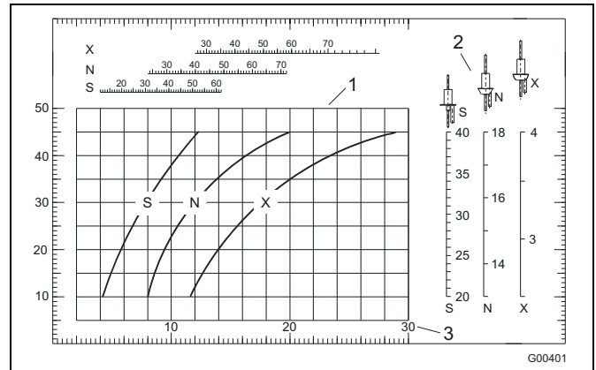
Fig. 3: Flowrate as a function of float shape and weight (example)
