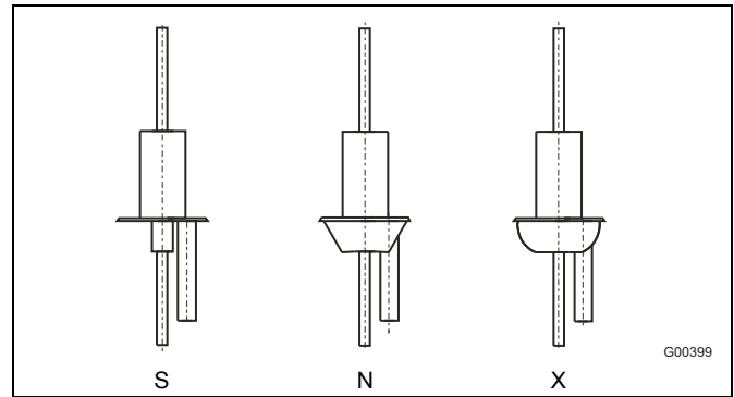
Fig. 2: Float shape overview
