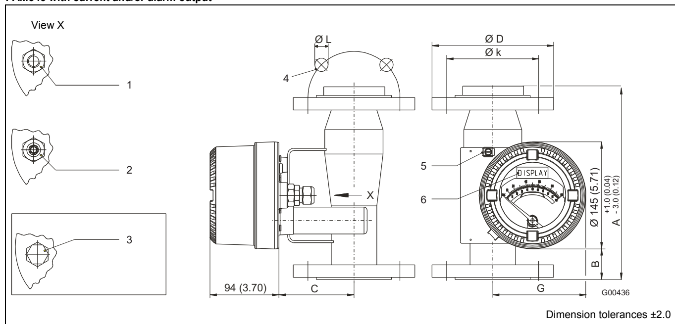
Fig. 22: All dimensions in mm (inch)
