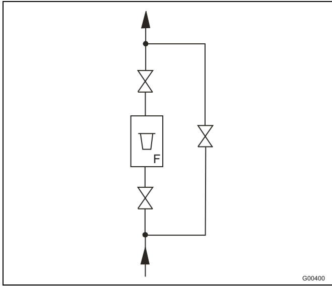
Fig. 1: Flowmeter installation
