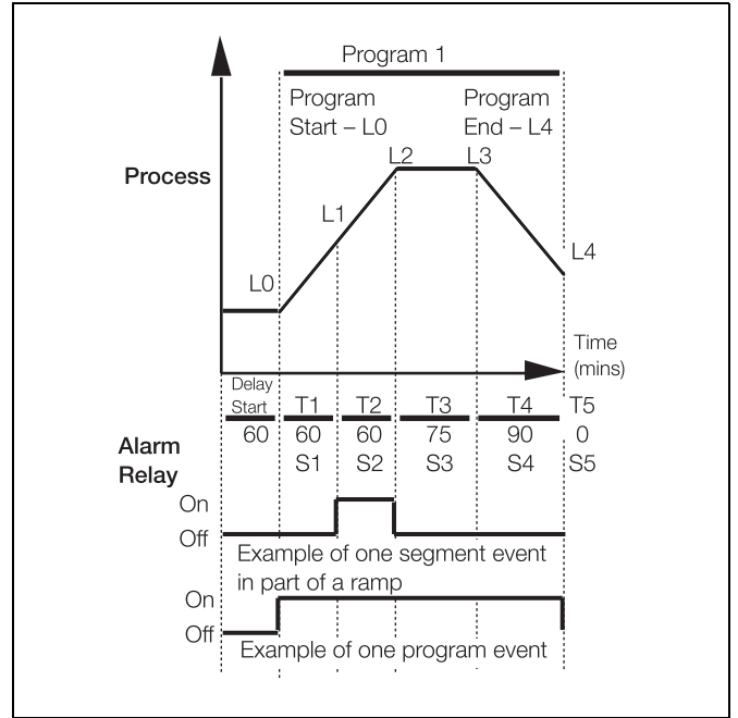
Ramp/Soak Program with Time Event Relay Sequences
