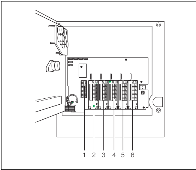
Module Positions
