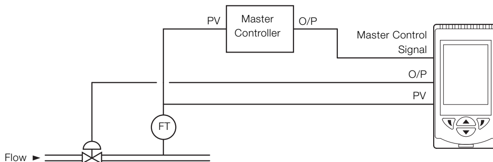
Fig. 15: Auto / Manual station and analog backup station
