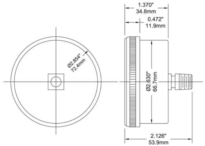
2.5" Back Connection
