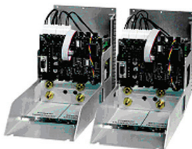
Up to two separate controller modules (channel: A and B) per instrument
